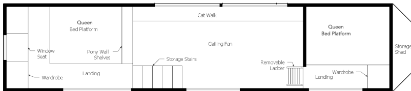
36' x 8.5' Bunkhouse Floor Plan with 3 Stand-Up Sleeping Areas
